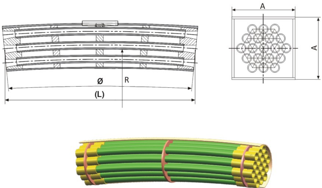
Individual strand deviator data
