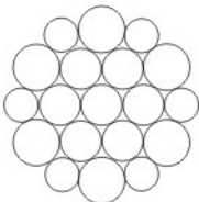
Cross-section of 28mm strand
