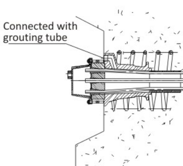
Step 8: Grouting
