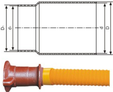
OLT coupler
