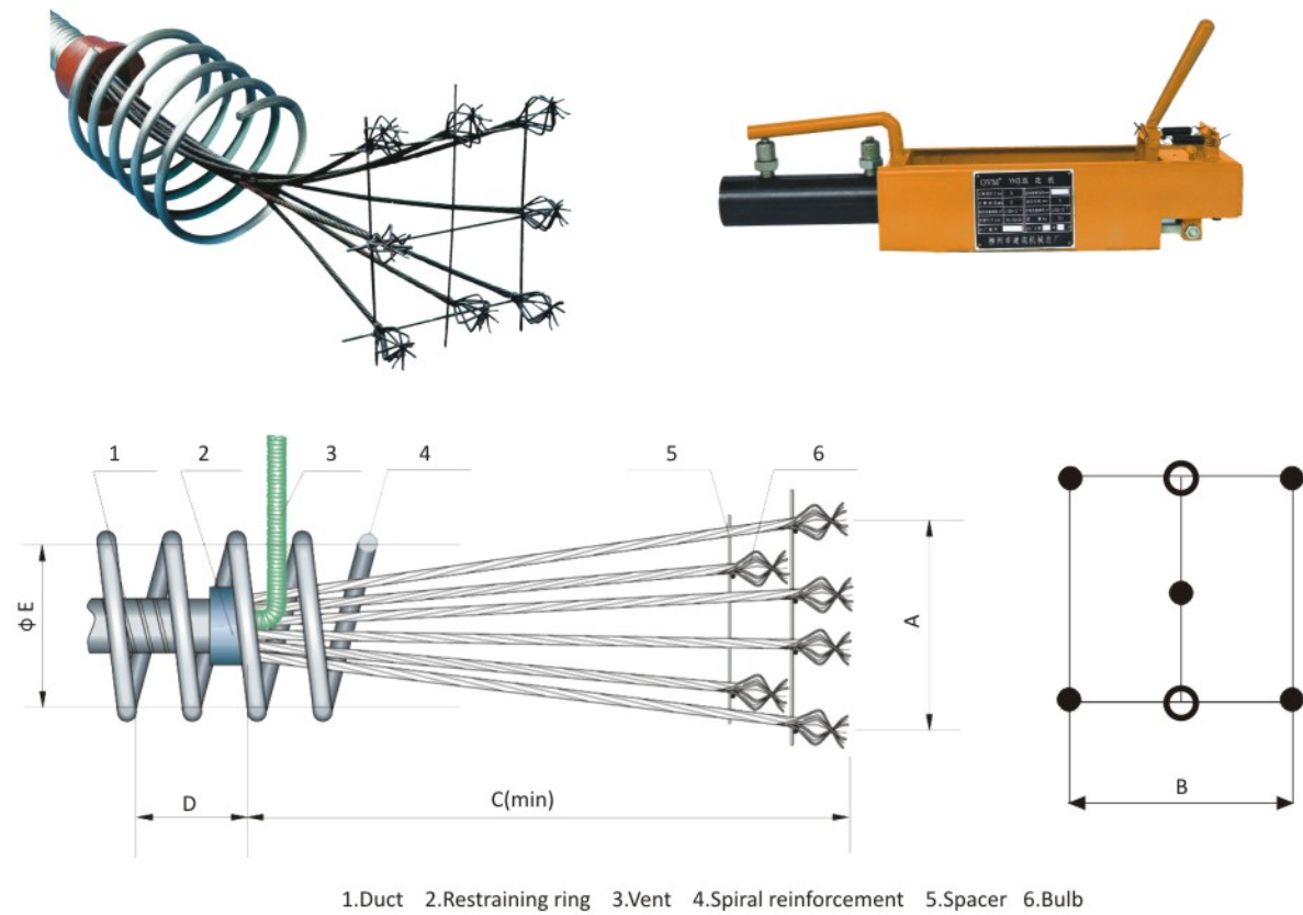
Main Data
