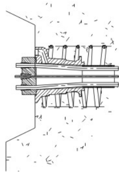
Step 7: Removal of jack and cutting of extra strand
