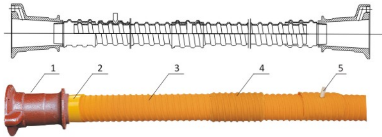
1.Bearing plate 2.OLT coupler 3.Plastic duct 4.OLG coupler 5.Vent
