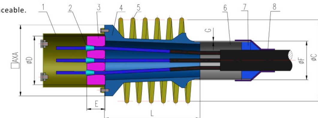
Type OVM.TS External Prestressing Anchorage Diagram
