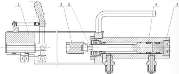
1.Jack 2.Pushing head 3.Piston 4.Cylinder
