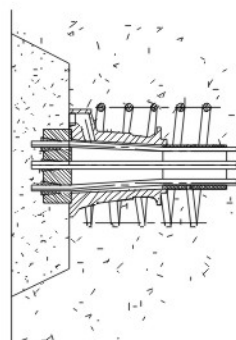
Step 9: Anchorage sealing
